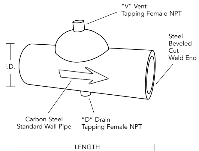
STANDARD SIZES 3" TO 24" • AVAILABLE UP TO 48" DIAMETER • Please consult factory for end fitting configurations
