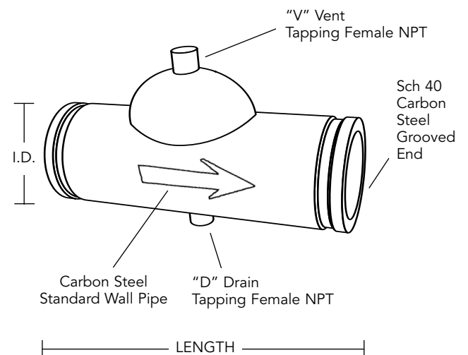
STANDARD SIZES 3" TO 24" • AVAILABLE UP TO 48" DIAMETER • Please consult factory for end fitting configurations
